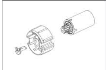
Picture 2: Coupling locking device
