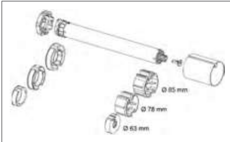
Picture 1: Examples for different shaft sizes
